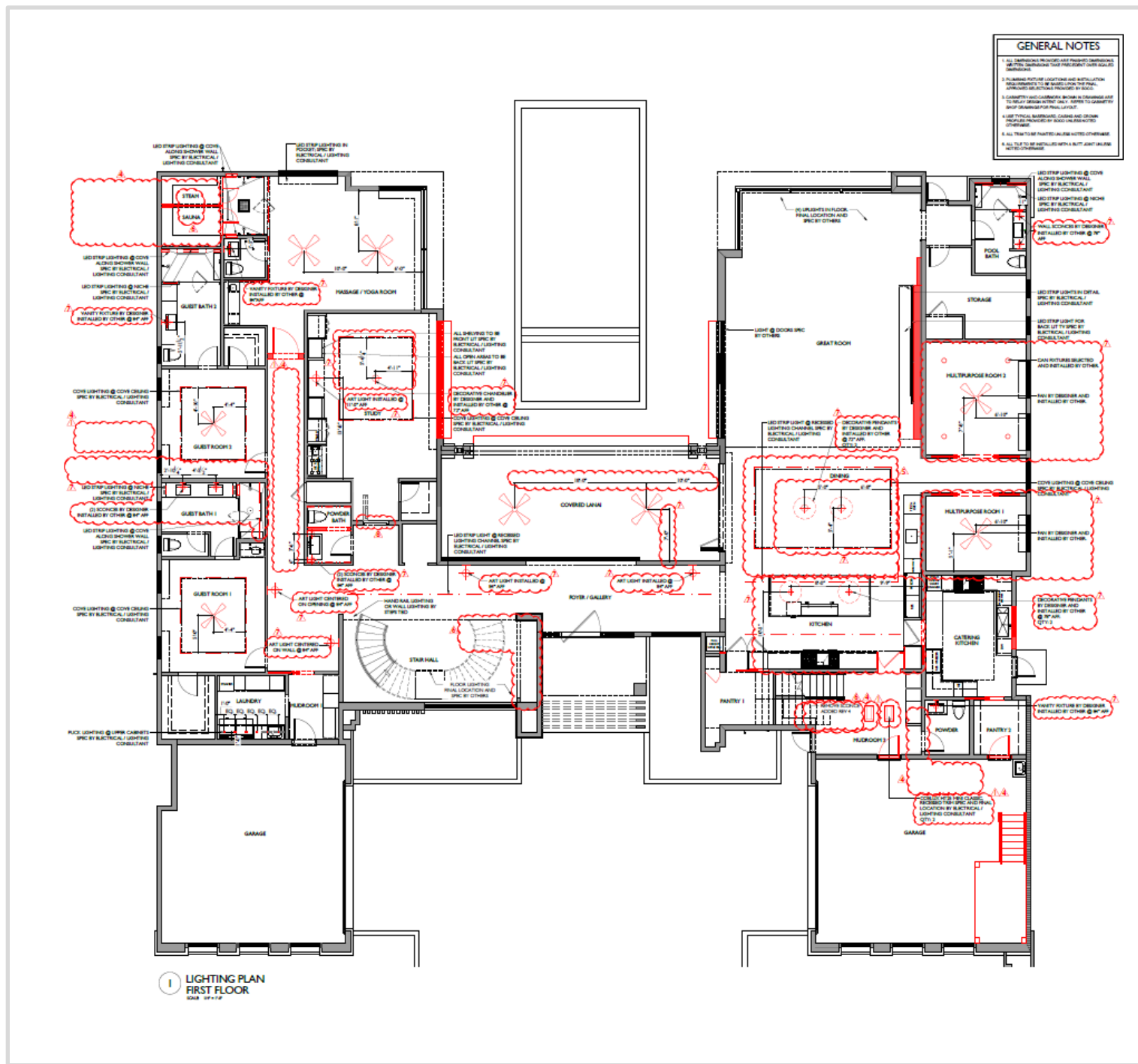
FIRST FLOOR
