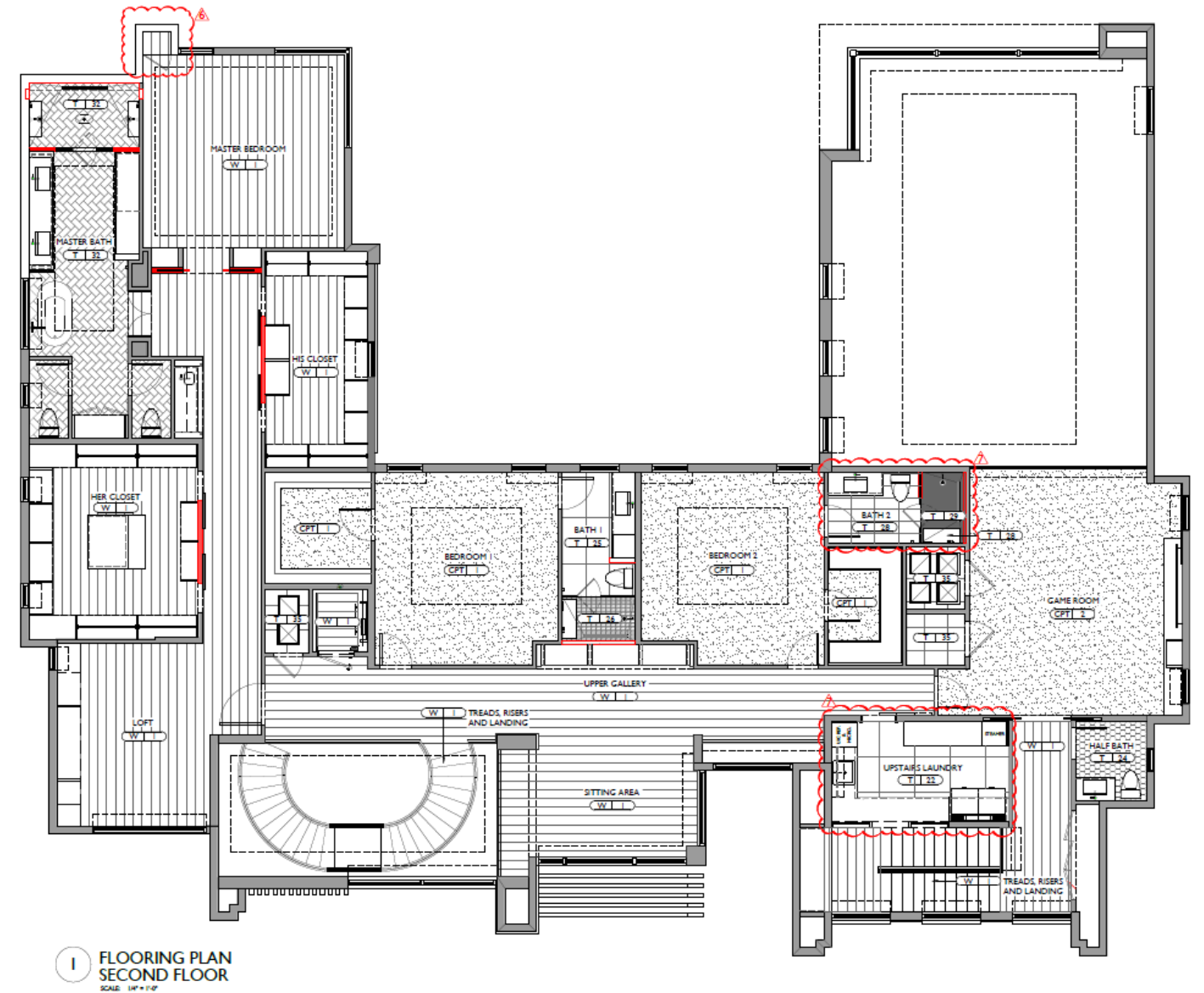
SECOND FLOOR
