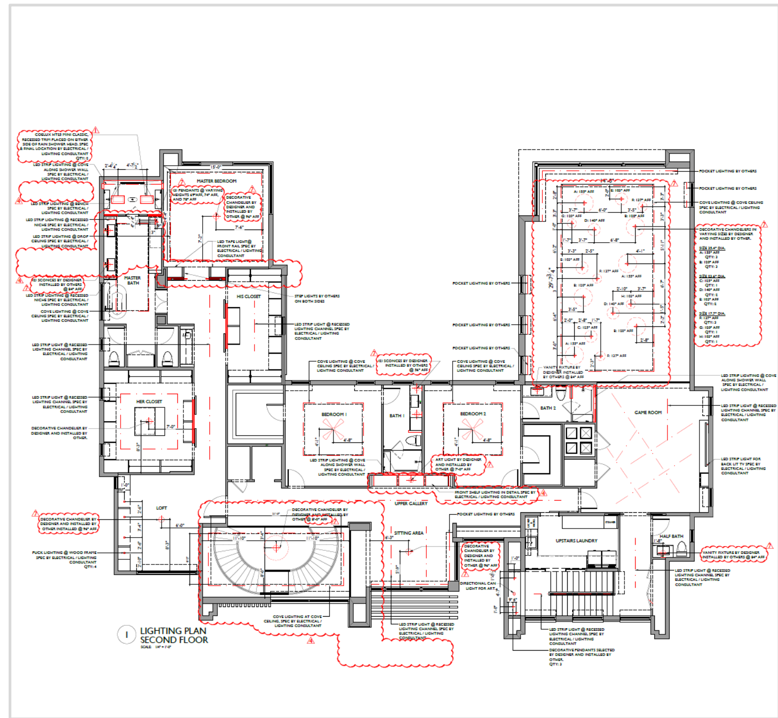
SECOND FLOOR
