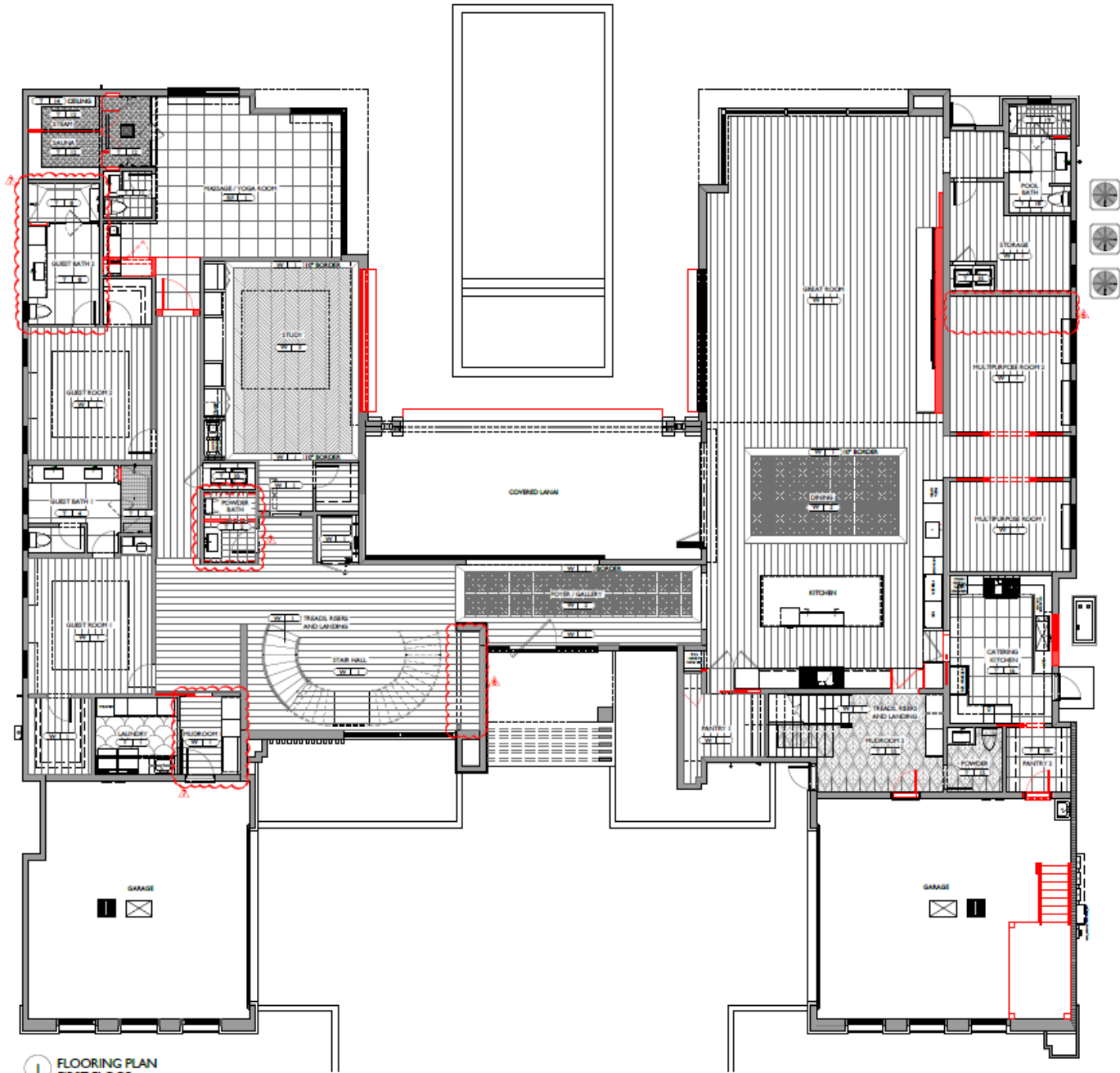
FIRST FLOOR
