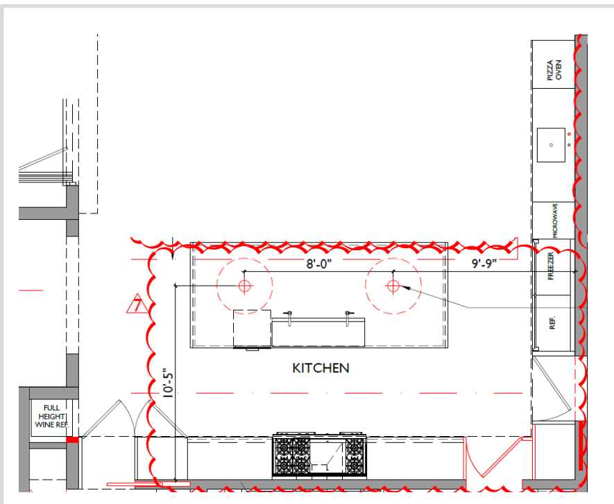
LIGHTING PLAN
