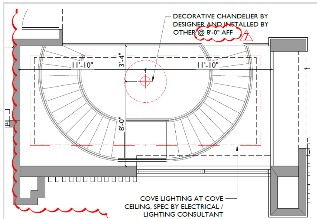
LIGHTING PLAN
