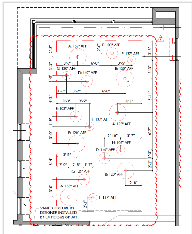
LIGHTING PLAN
