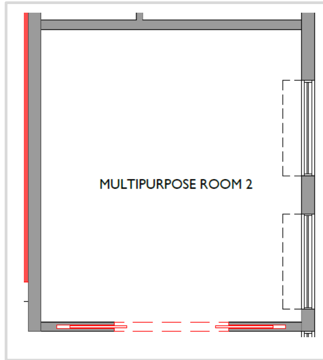
FLOOR PLAN
