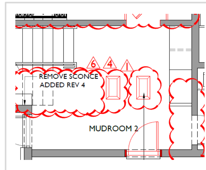
LIGHTING PLAN
