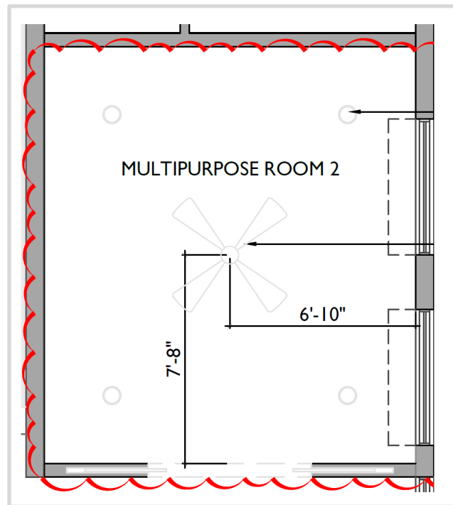
LIGHTING PLAN
