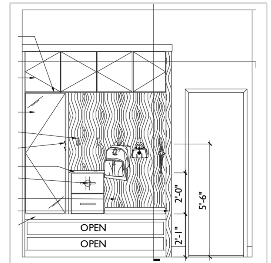
ELEVATION OF MUDROOM BUILT-IN
