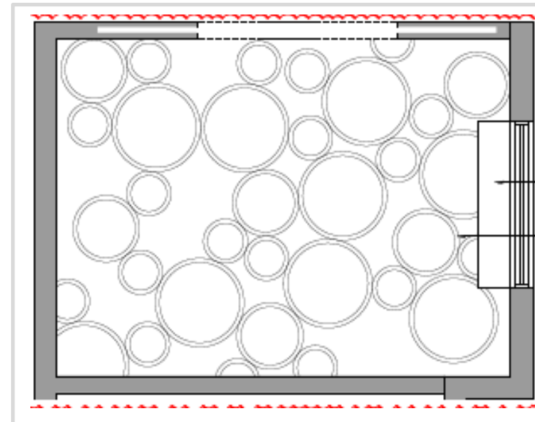
CEILING DETAIL
