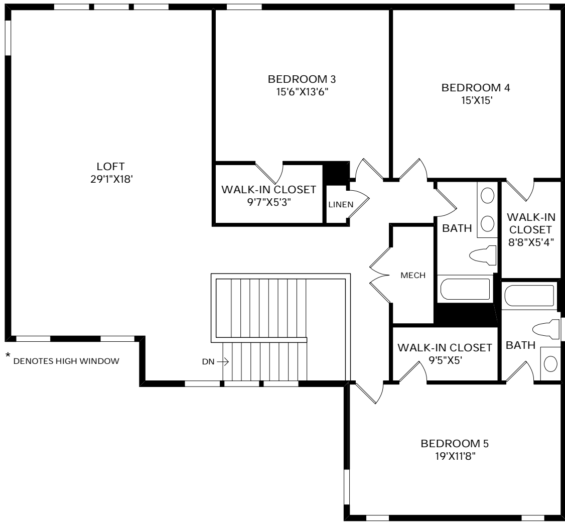
SECOND FLOOR 9' CEILING HEIGHT
